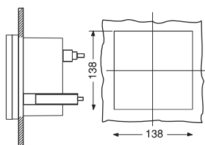
Rear panel mounting
