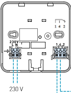
230V POWER SUPPLY
